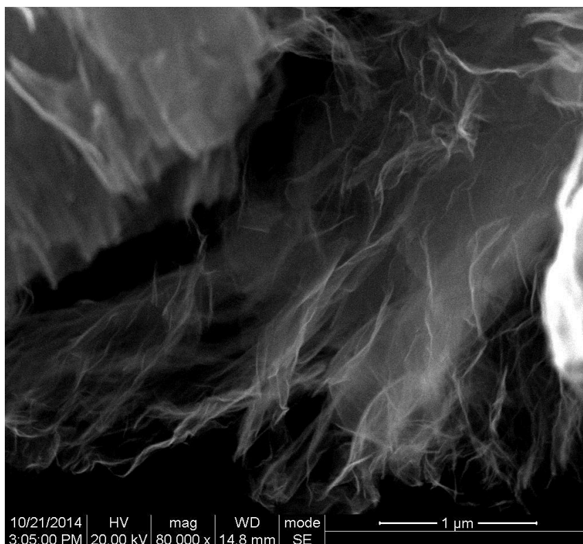
SEM of Graphene NMP Paste
